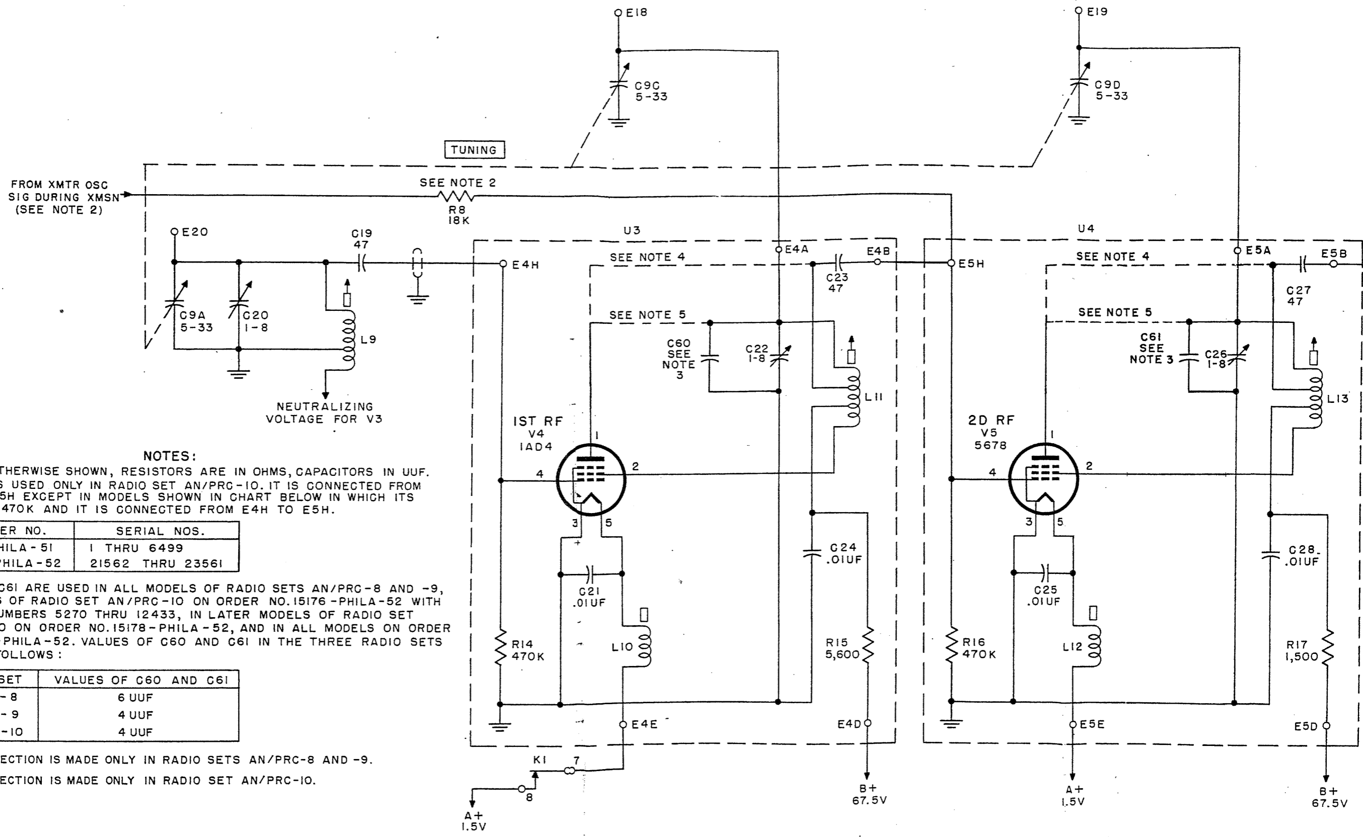
Figure 5. Rf amplifier circuits.
