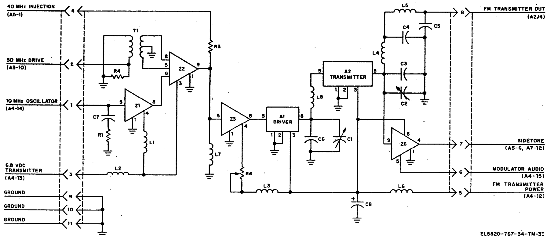
Figure 4-13. FM transmitter module A6 schematic diagram.
