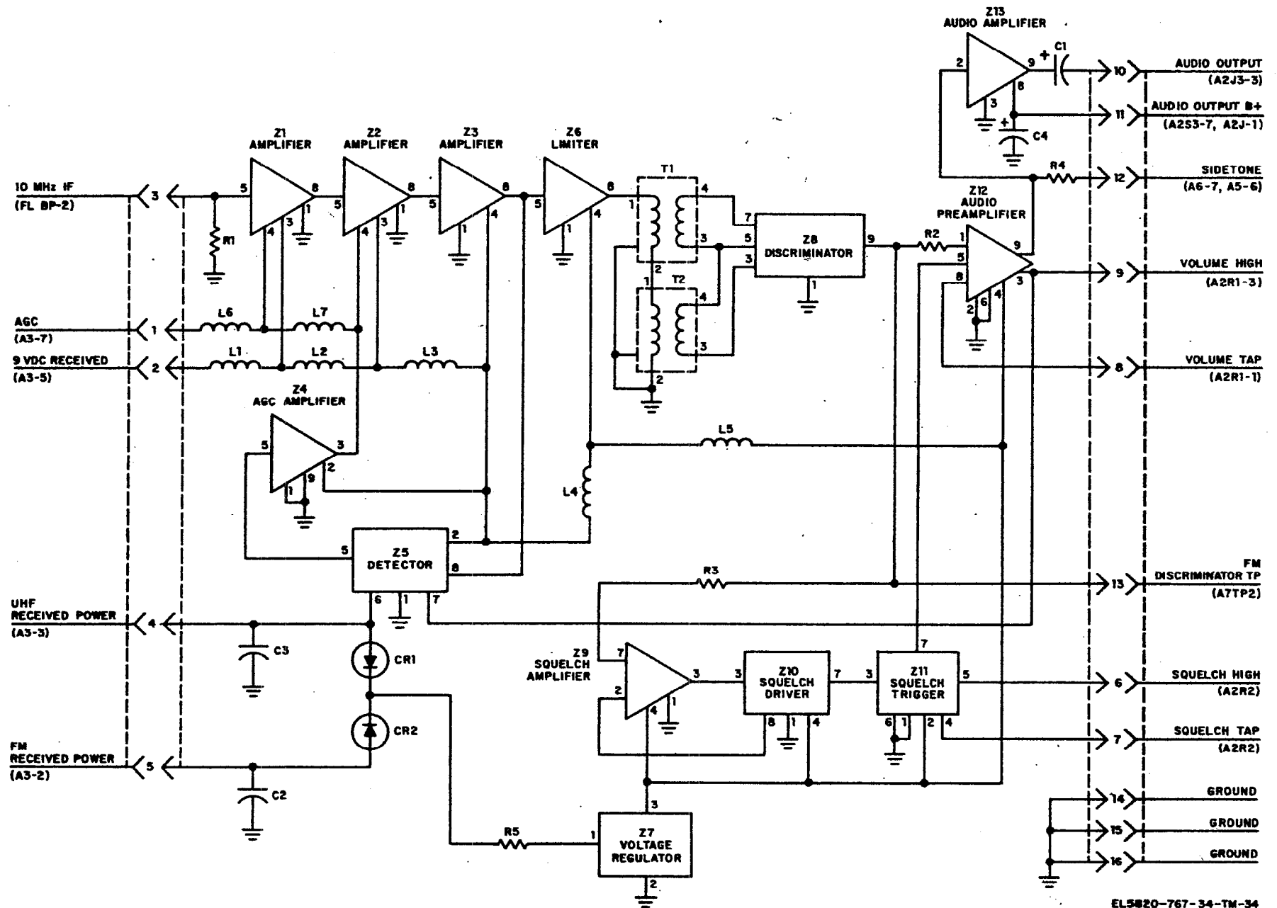
Figure 4-14. If.-af amplifier module A7 schematic diagram.
