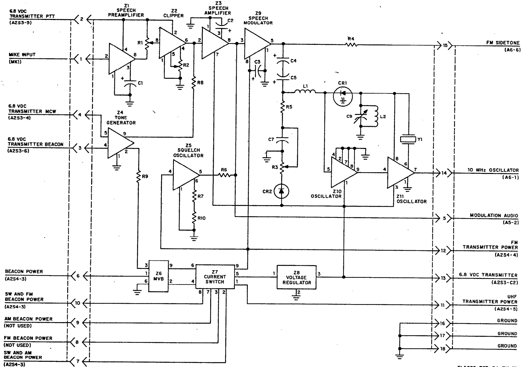
Figure 4-11. Modulator module A4 schematic diagram.
