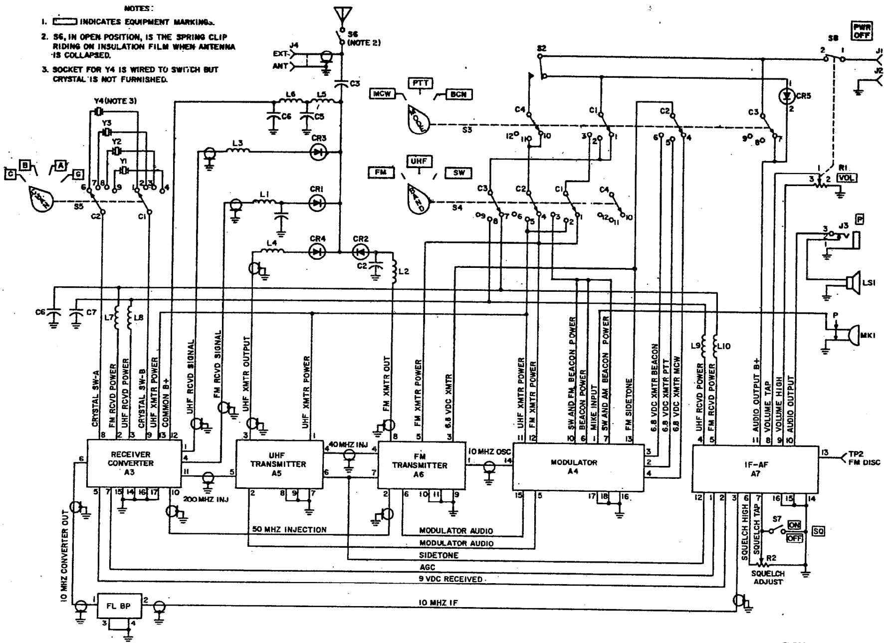
Figure 4-9. Radio Set AN/URC-68 schematic diagram.
