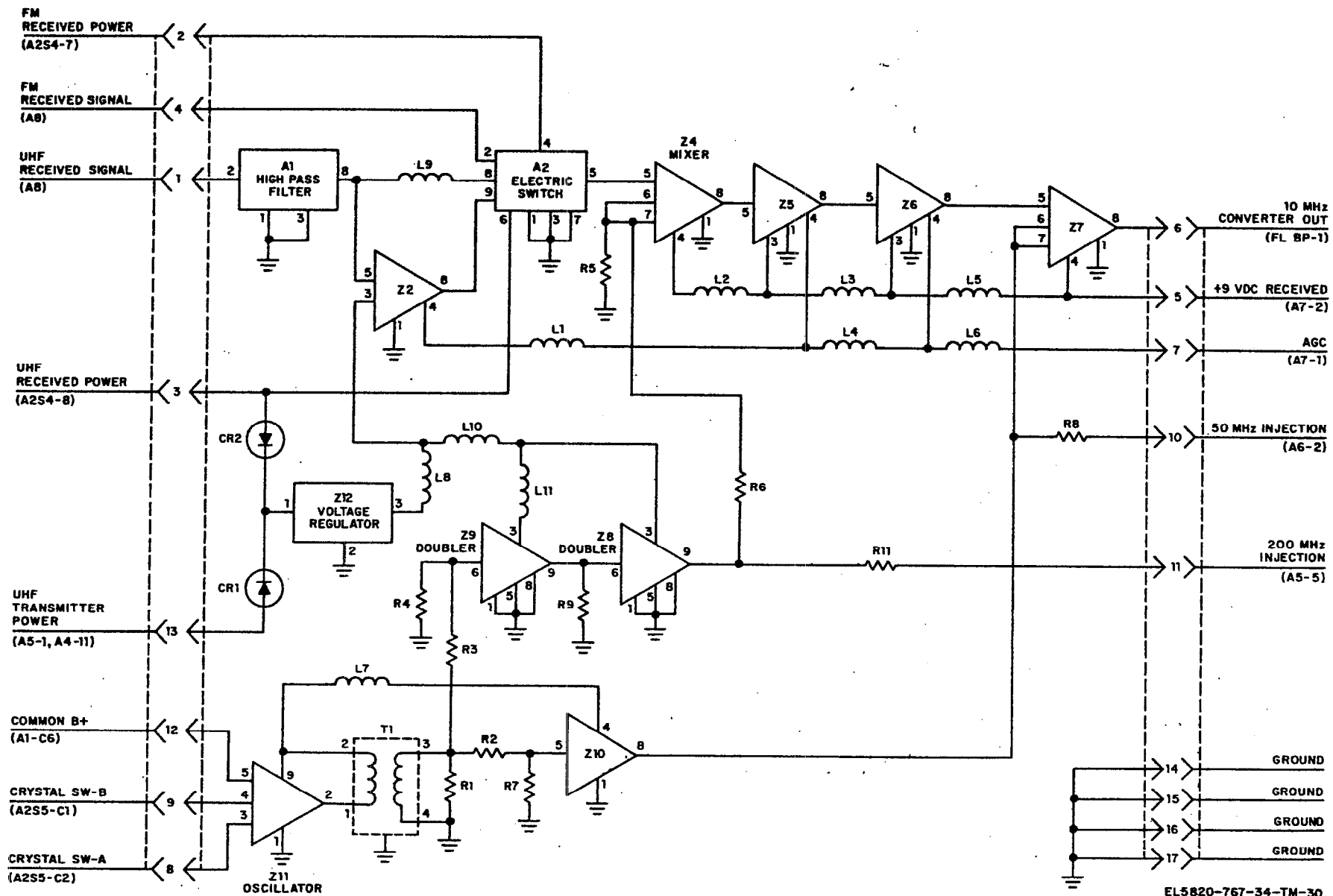
Figure 4-10. Receiver-converter module A3, schematic diagram.
