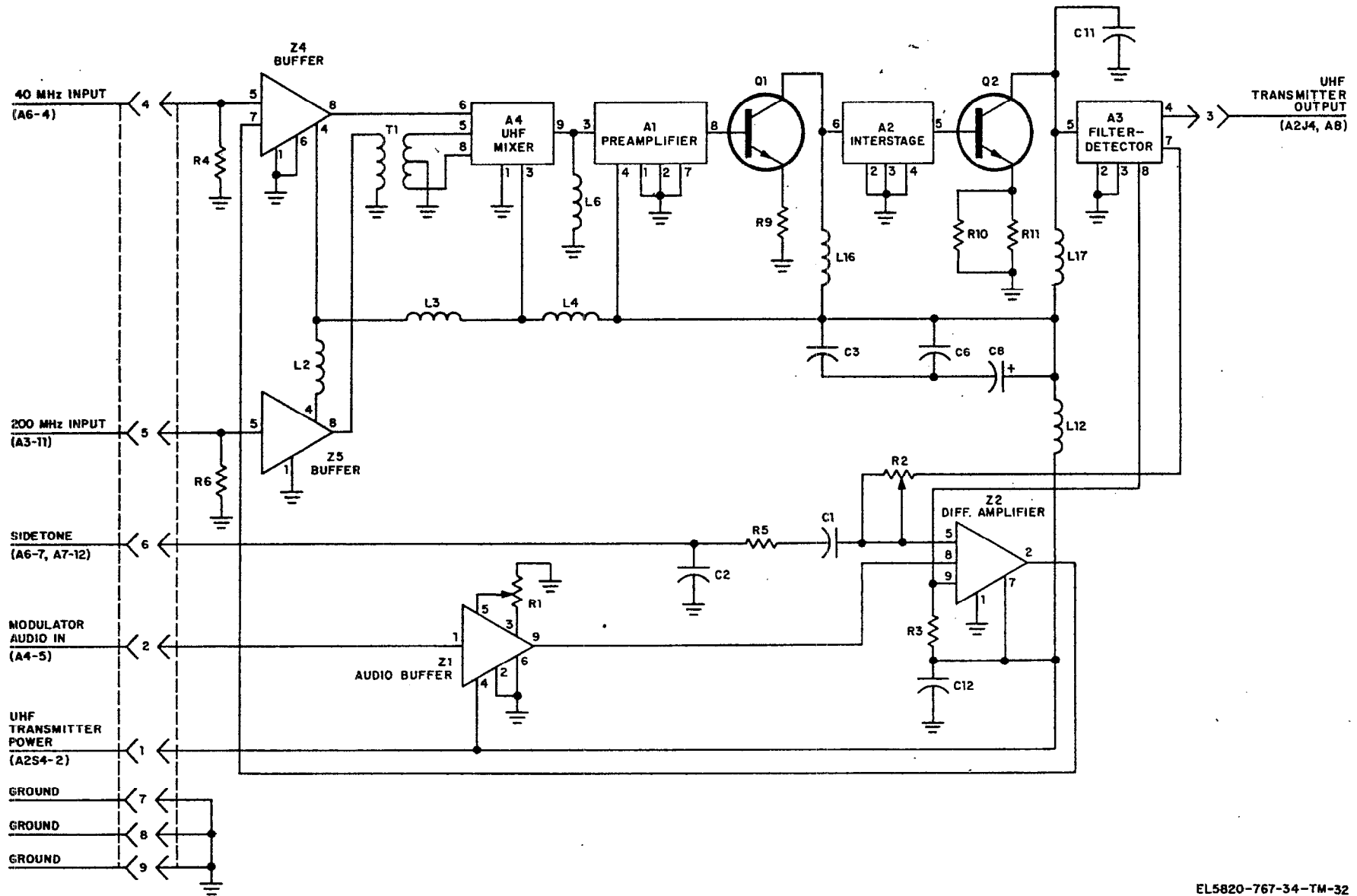
Figure 4-12. Uhf transmitter module A5 schematic diagram.
